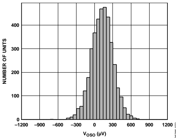
Figure 7. Typical Distribution of Output Offset Voltage
