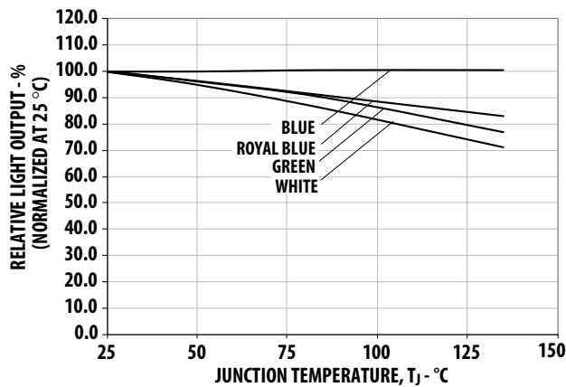
Figure 23 Relative Light Output vs. Junction Temperature
