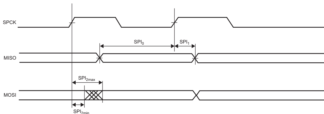
Figure 63-24. Minimum and Maximum Access Time for SPI Output Signal
