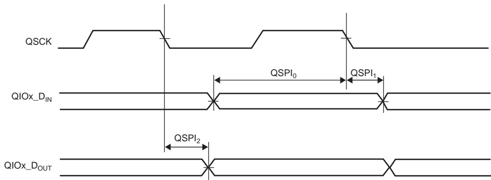
Figure 63-26. QSPI Master Mode 1
