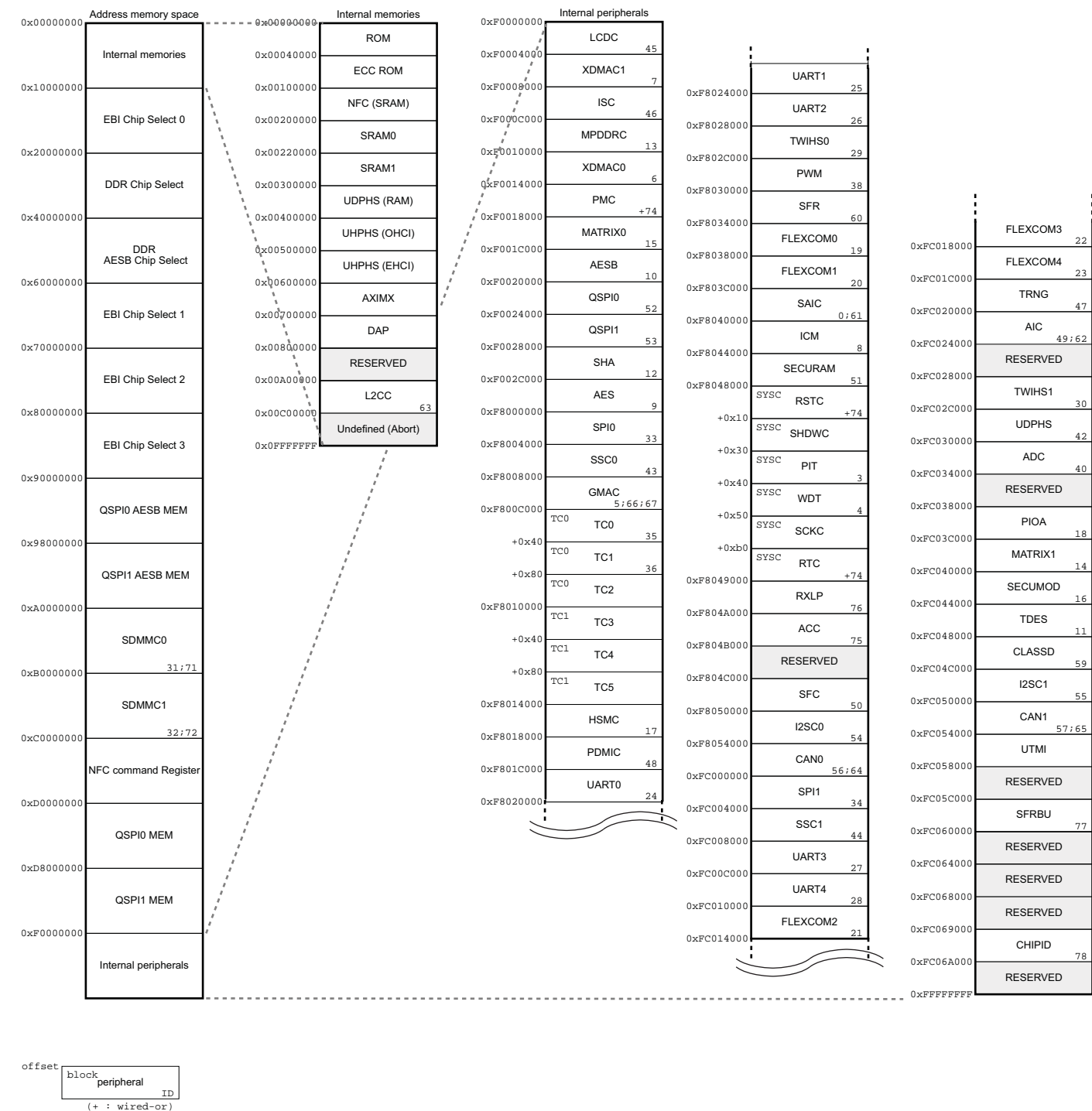
Figure 7-1. Memory Mapping
