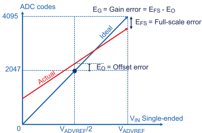
Figure 63-6. Gain and Offset Errors in Single-ended Mode
