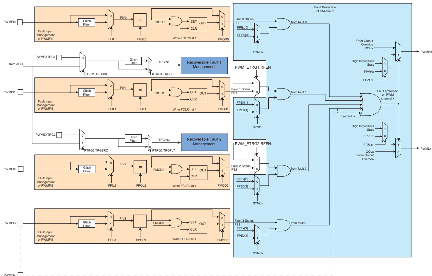
Figure 53-16. Fault Protection
