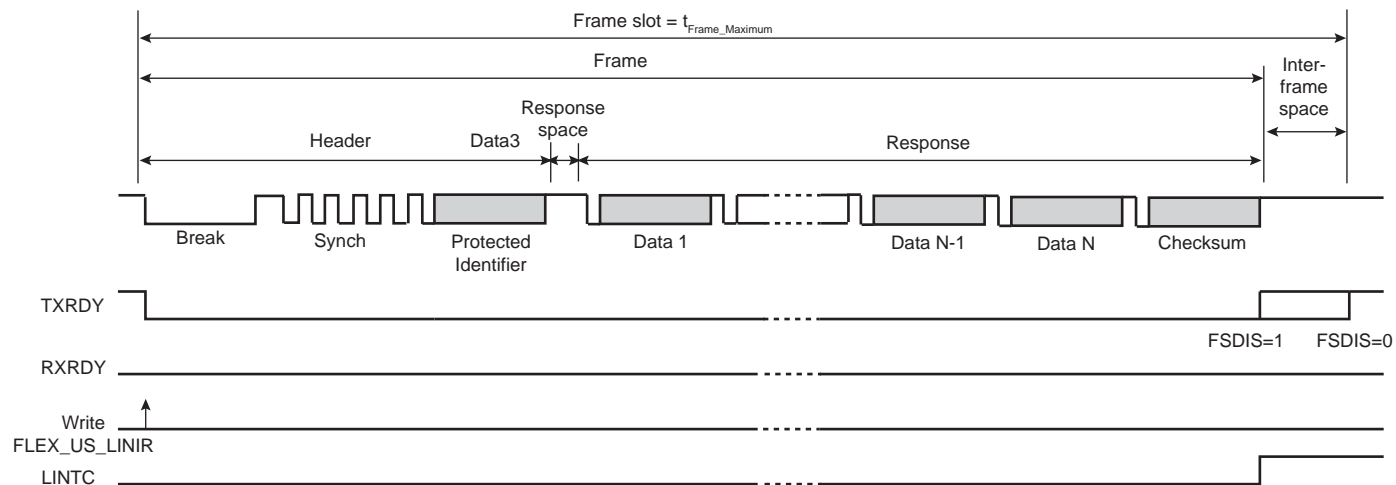
Figure 44-49. Master Node Configuration, NACT = IGNORE
