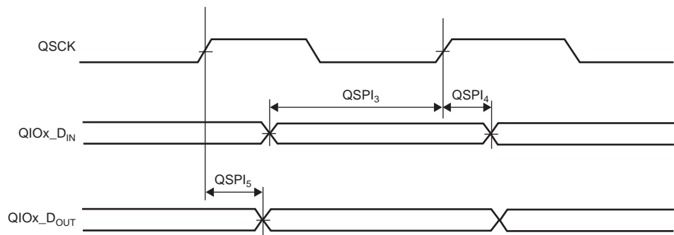
Figure 63-26. QSPI Master Mode 1
