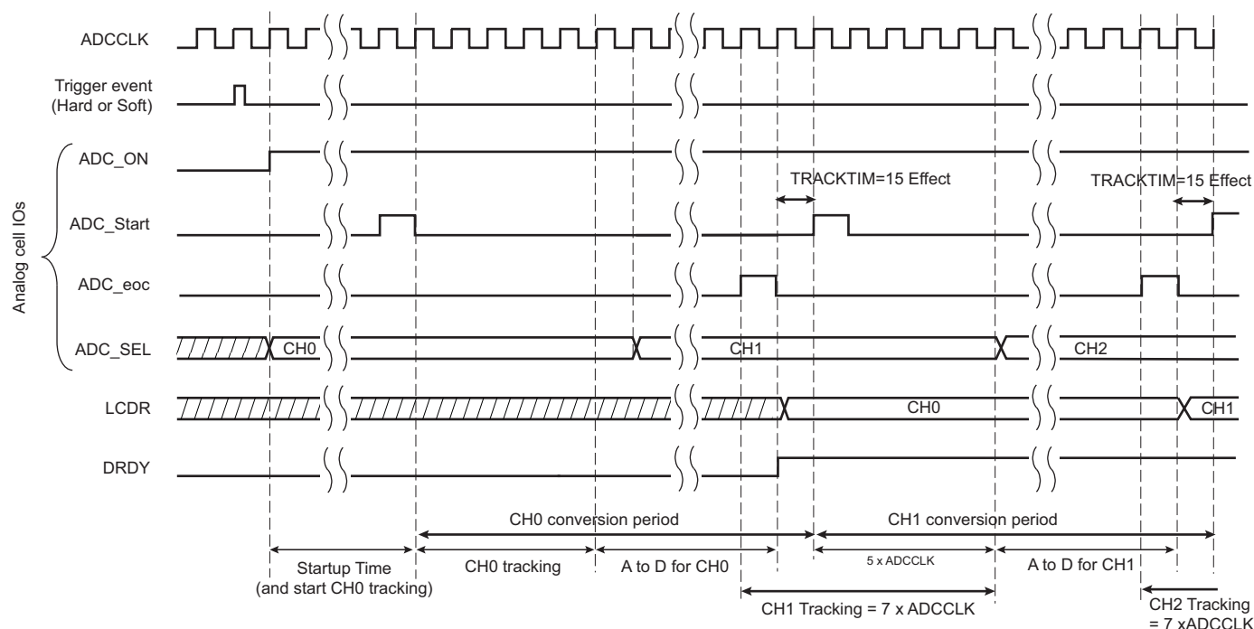
Figure 62-3. Sequence of Consecutive ADC Conversions with TRACKTIM = 15
