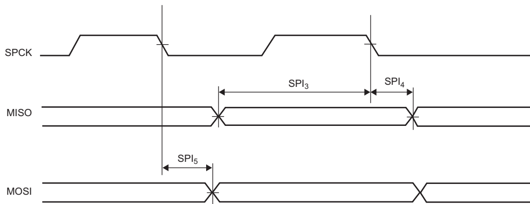
Figure 63-14. SPI Master Modes 0 and 3
