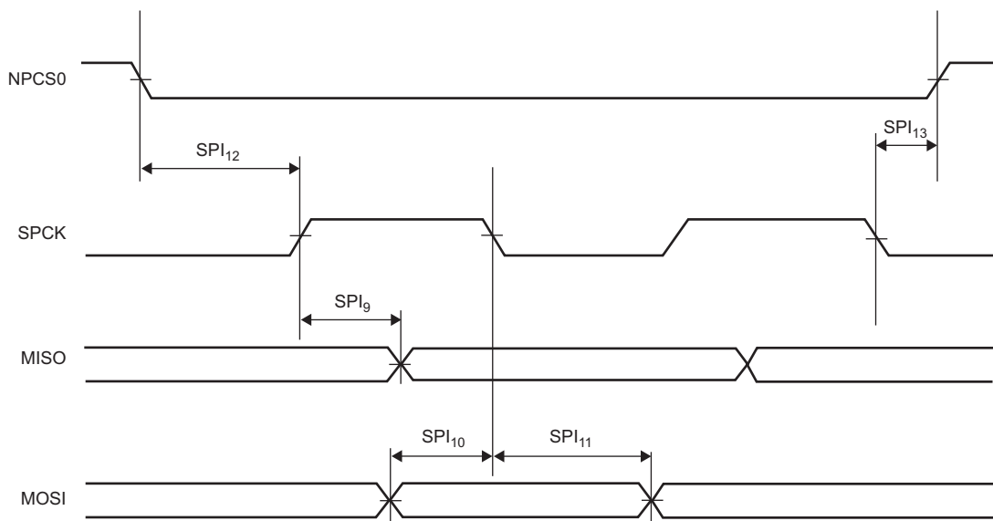
Figure 63-16. SPI Slave Modes 1 and 2
