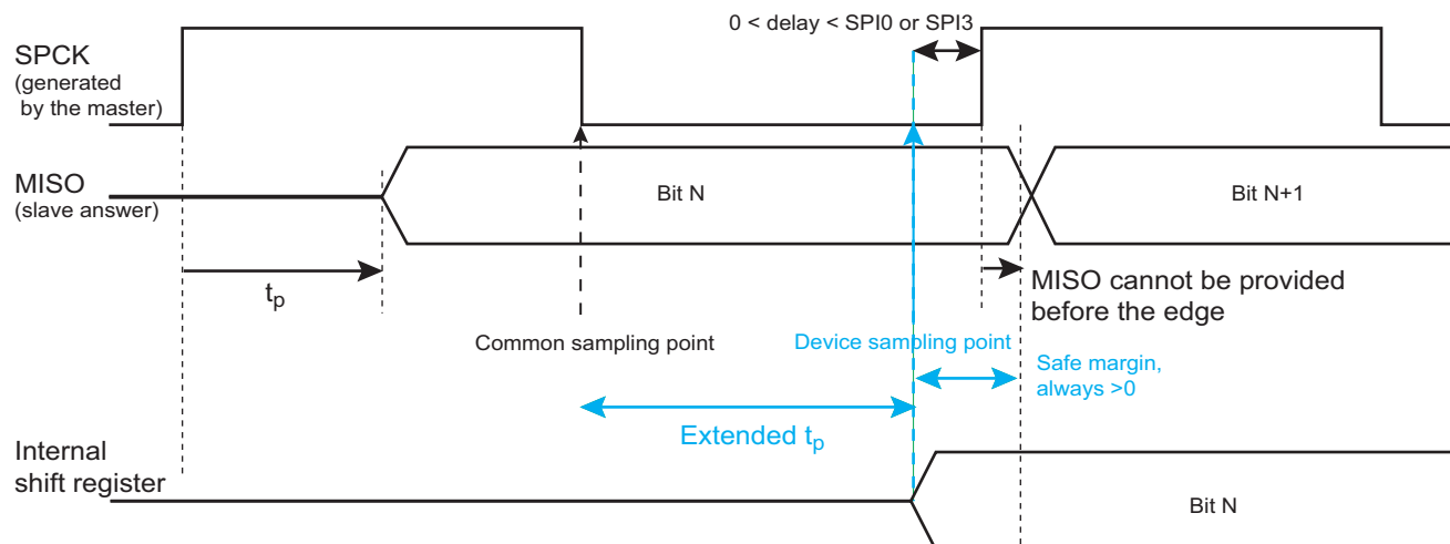
Figure 63-12. MISO Capture in Master Mode
