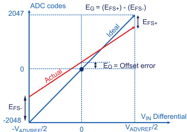
Figure 63-5. Gain and Offset Errors in Differential Mode
