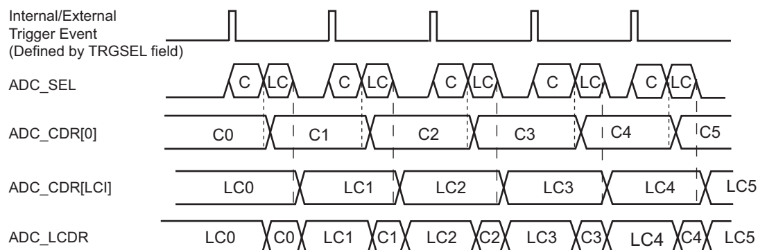
Figure 62-8. Same Trigger for All Channels (ADC_CHSR[LCI] = 1 and ADC_TRGR.TRGMOD = 1, 2, 3, 5)
