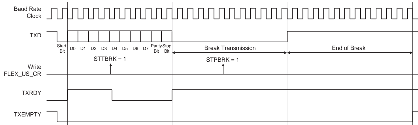
Figure 44-25. Break Transmission
