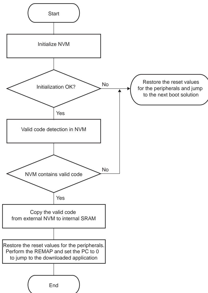
Figure 15-4. NVM Boot Diagram
