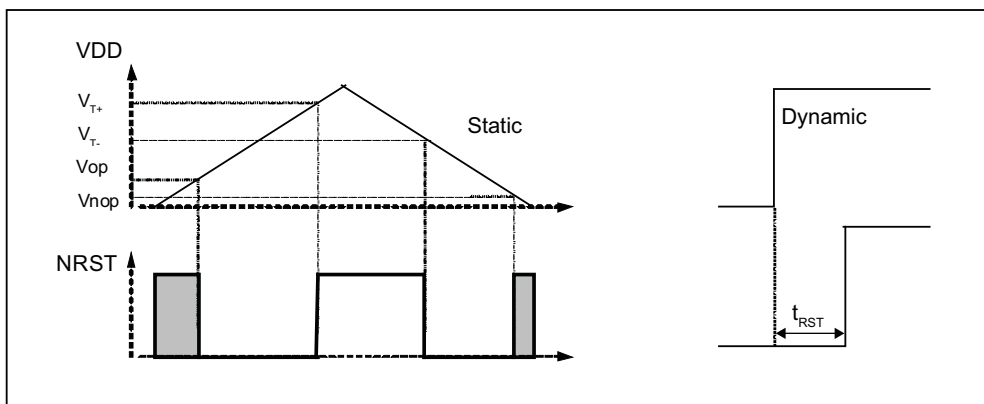
Figure 63-9. General Presentation of POR Behavior
