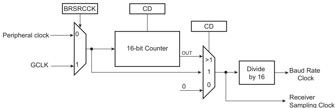
Figure 45-3. Baud Rate Generator
