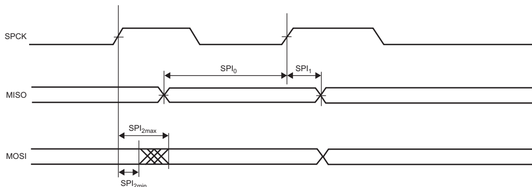
Figure 63-18. Minimum and Maximum Access Time for SPI Output Signal
