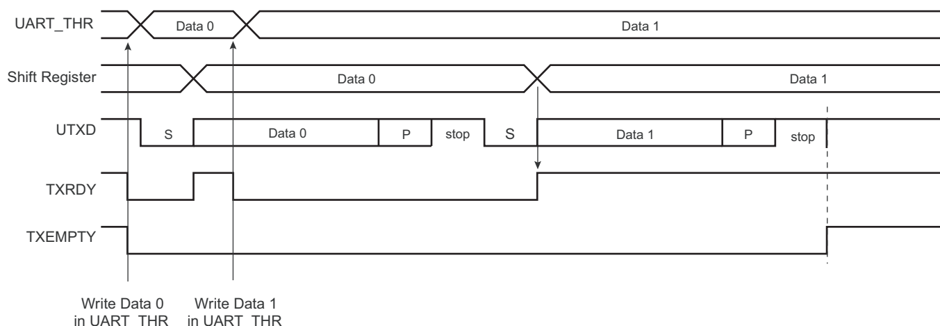
Figure 45-12. Transmitter Control
