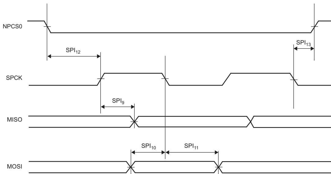
Figure 63-22. FLEXCOM in SPI Slave Modes 1 and 2
