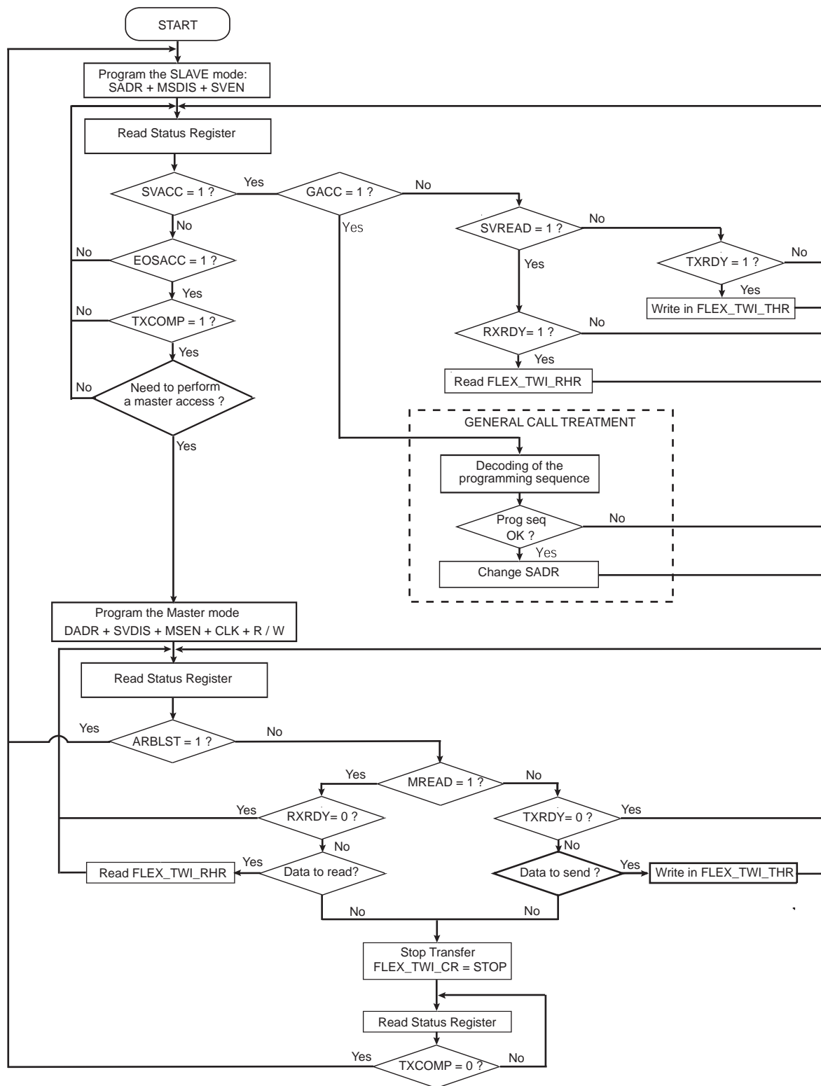
Figure 44-117. Multi-Master Flowchart
