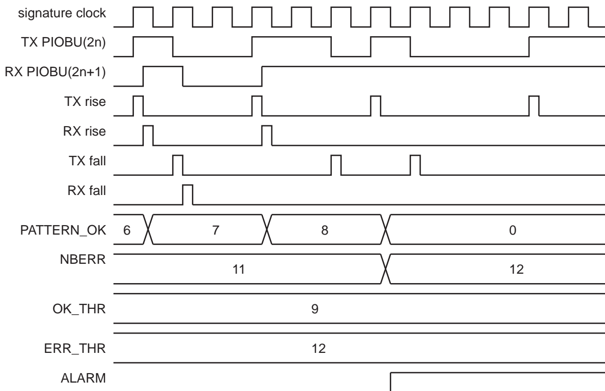
Figure 61-10. Dynamic Signatures: Raising Alarm After Receiving a Sufficient Number of Bad Patterns
