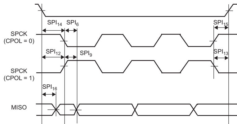
Figure 63-17. SPI Slave Mode - NPCS Timings
