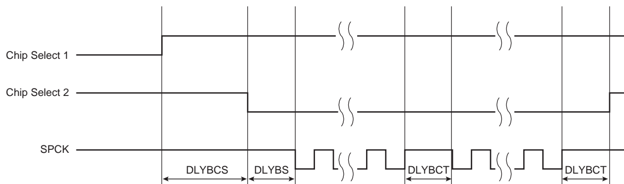
Figure 46-9. Programmable Delays
