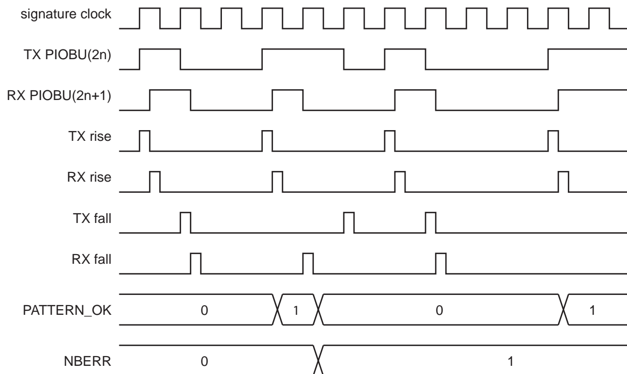
Figure 61-8. Dynamic Signature Ongoing, One Error
