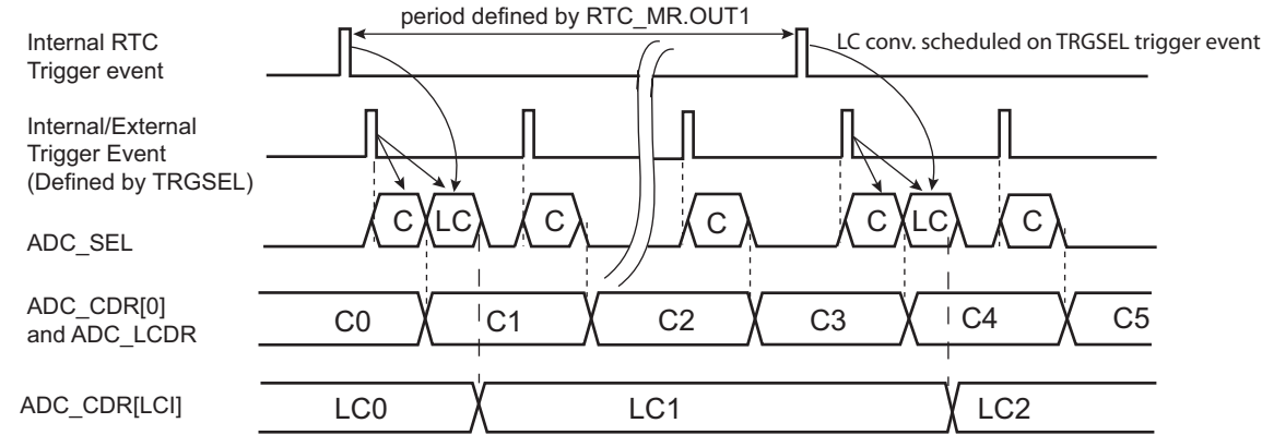
Figure 62-9. Independent Trigger Measurement for Last Channel (ADC_CHSR[LCI] = 0 and ADC_TRGR.TRGMOD = 1, 2, 3, 5)
