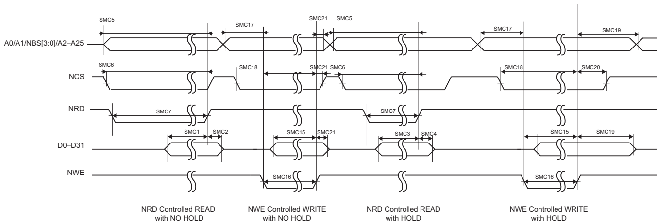
Figure 63-11. SMC Timings - NRD Controlled Read and NWE Controlled Write
