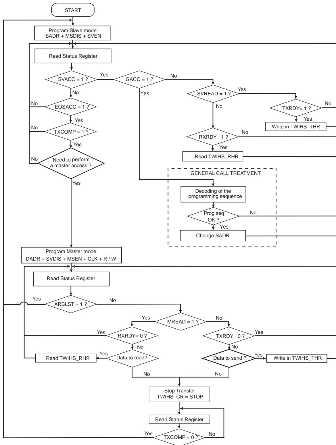
Figure 43-35. Multimaster Flowchart
