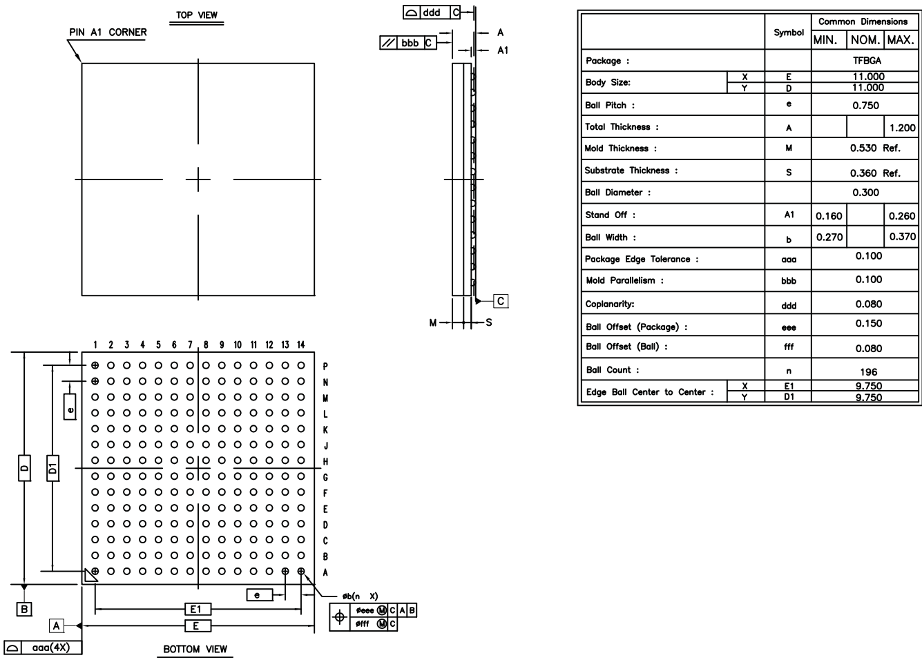
Figure 64-3. Mechanical Overview of the 196-ball TFBGA Package
