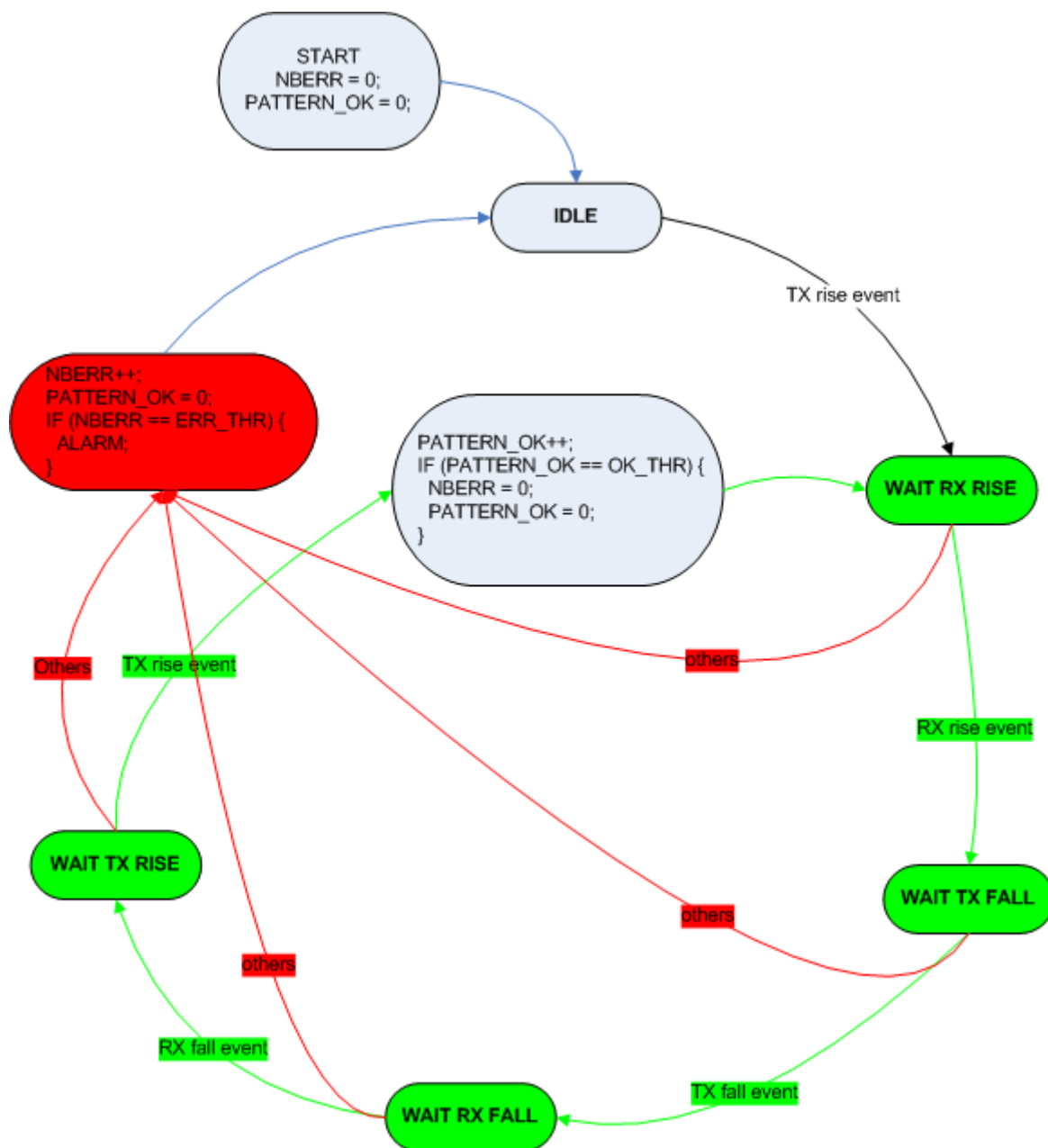
Figure 61-6. Dynamic Detection Mechanism State Machine
