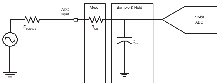
Figure 63-8. Simplified Acquisition Path
