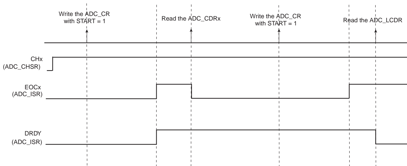
Figure 62-4. EOCx and DRDY Flag Behavior
