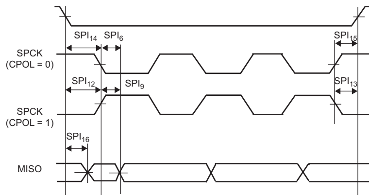
Figure 63-23. FLEXCOM in SPI Slave Mode - NPCS Timings
