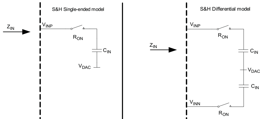
Figure 63-7. Input Channel Model
