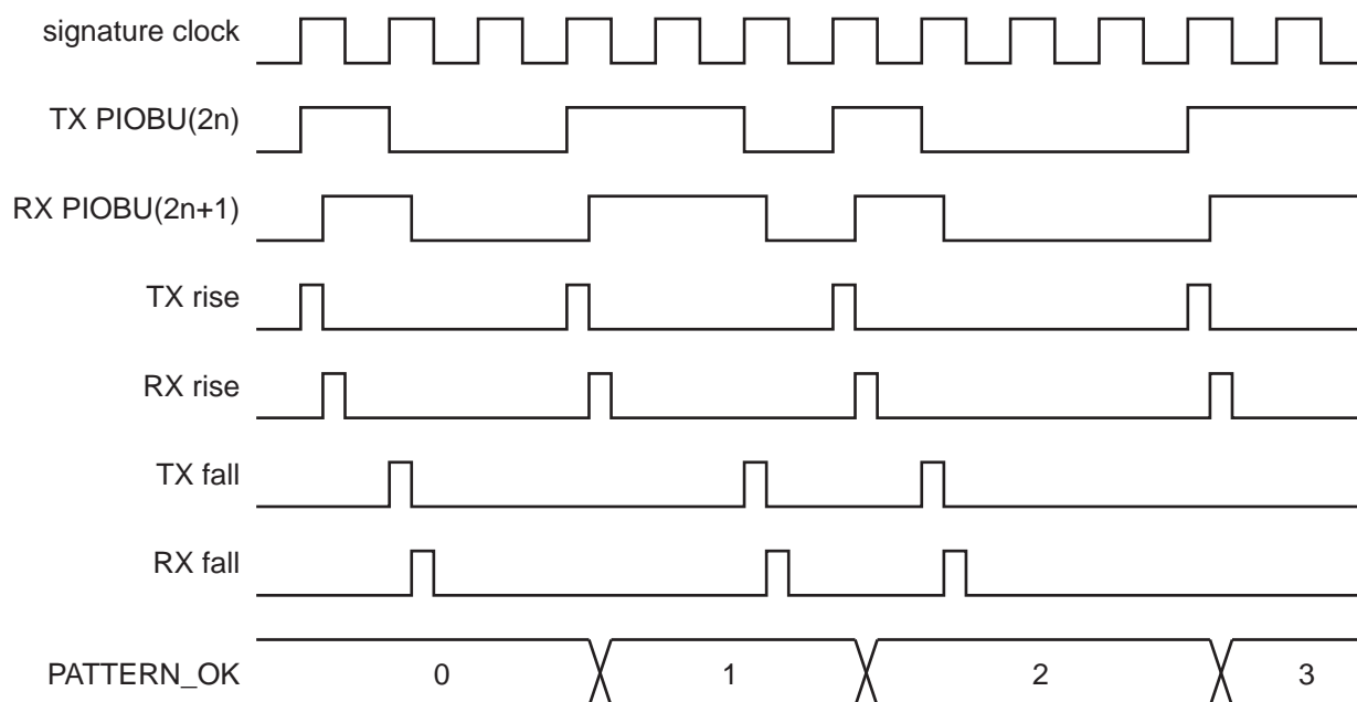
Figure 61-7. Dynamic Signature Ongoing, No Error
