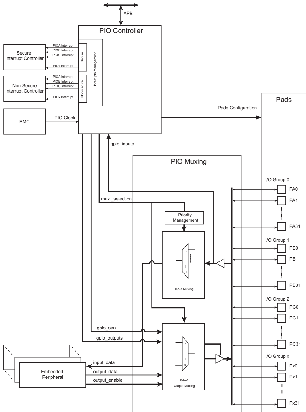
Figure 31-1. Block Diagram
