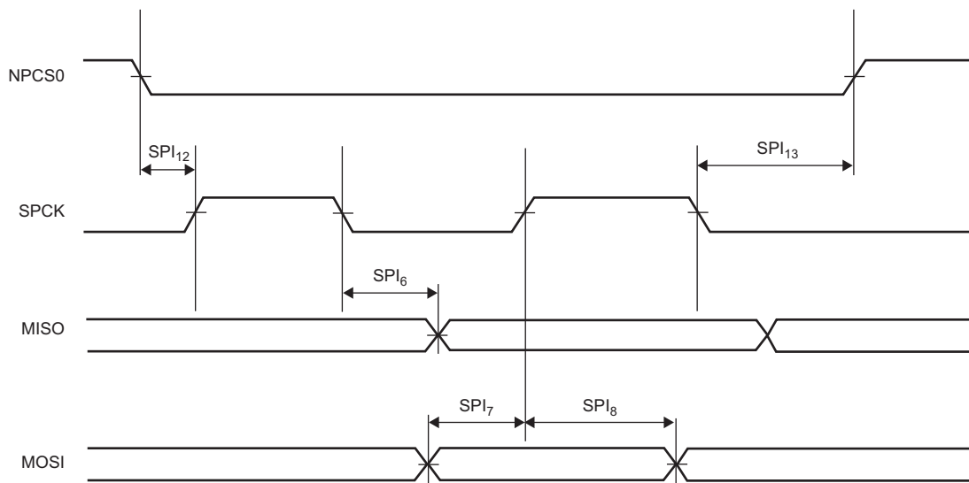
Figure 63-21. FLEXCOM in SPI Slave Modes 0 and 3
