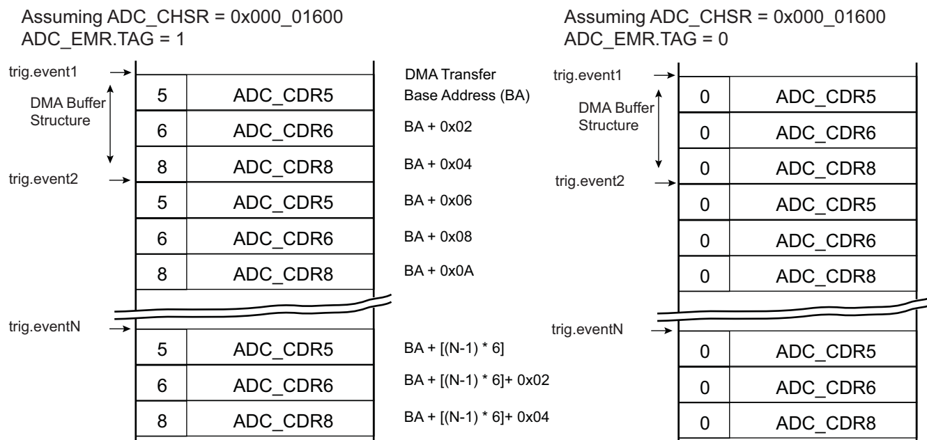
Figure 62-21. Buffer Structure
