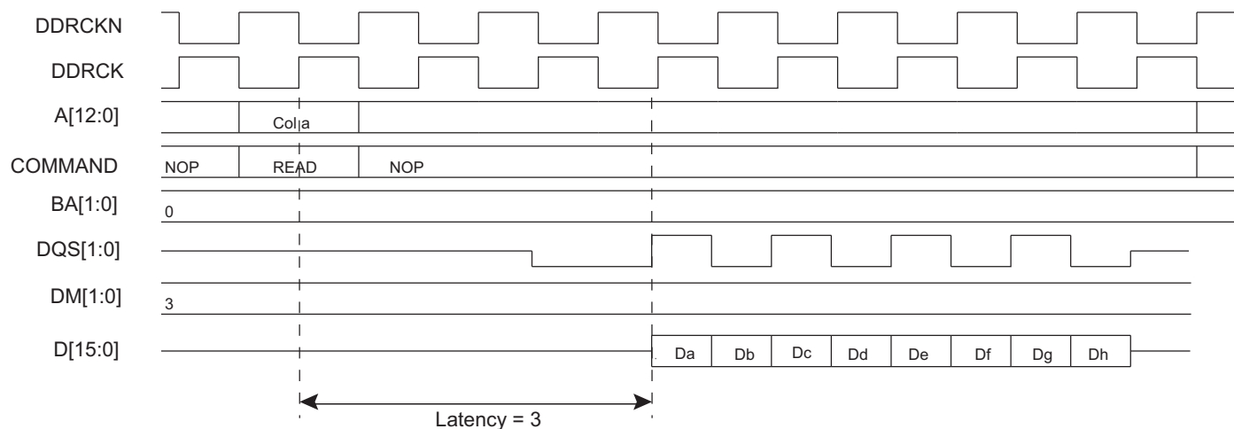
Figure 33-12. Burst Read Access, Latency = 3, DDR2-SDRAM Devices
