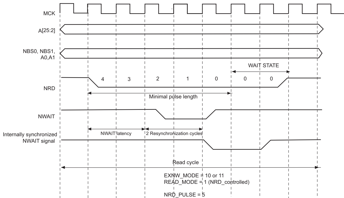
Figure 34-27. NWAIT Latency
