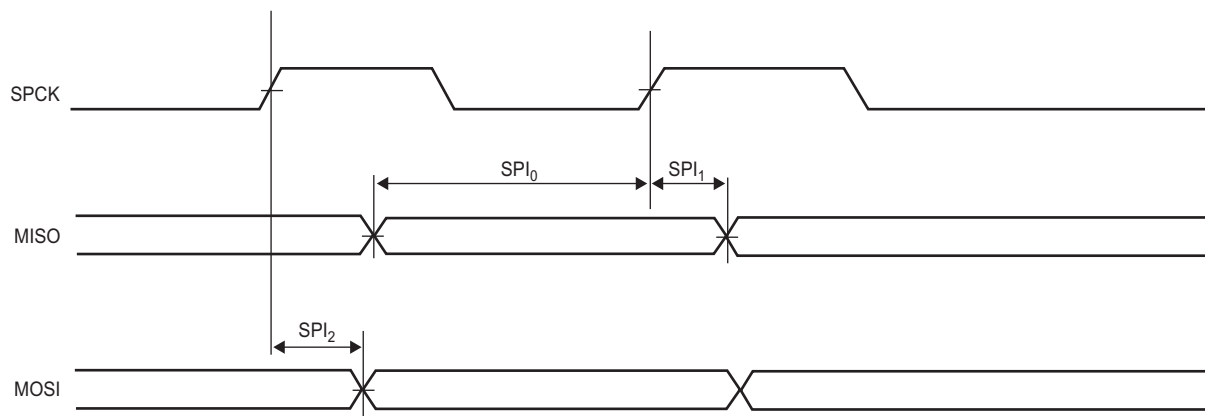
Figure 63-13. SPI Master Modes 1 and 2
