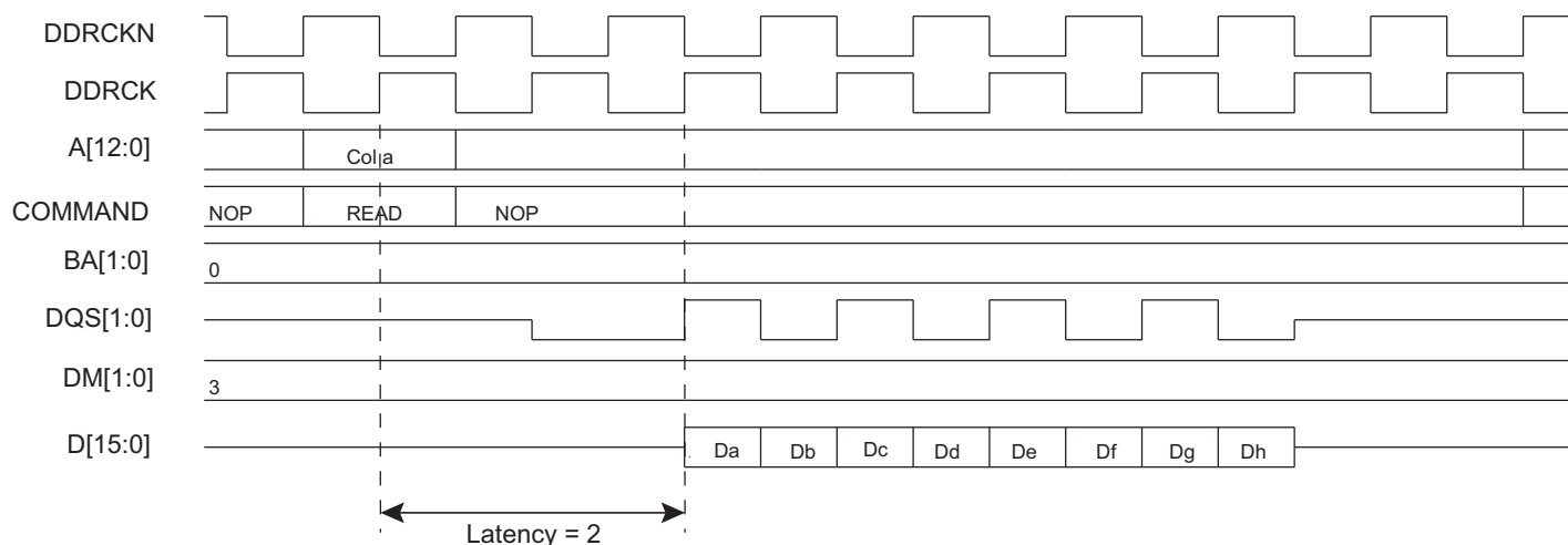
Figure 33-11. Burst Read Access, Latency = 2, DDR-SDRAM Devices
