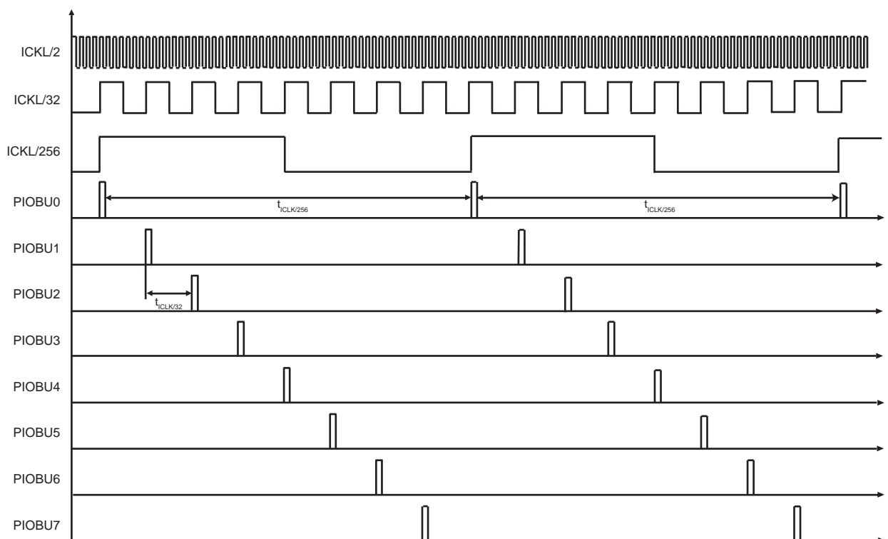
Figure 61-3. Schedule Principle
