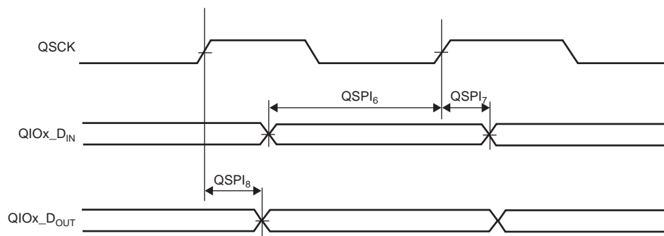
Figure 63-28. QSPI Master Mode 3
