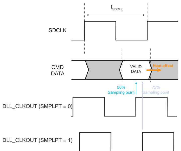
Figure 48-4. SDR104/HS200 Sampling Point Selection
