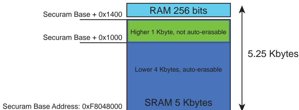
Figure 61-2. Security Module Internal Memory Map
