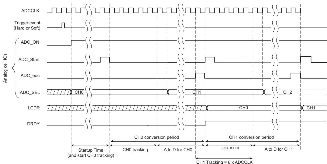
Figure 62-2. Sequence of Consecutive ADC Conversions with TRACKTIM = 0
