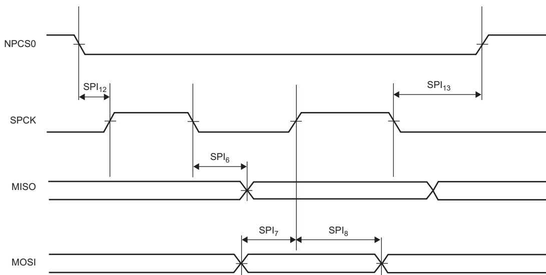
Figure 63-15. SPI Slave Modes 0 and 3
