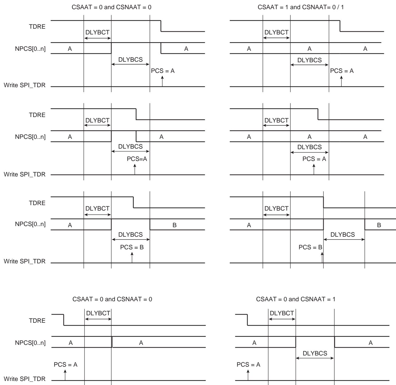
Figure 46-11. Peripheral Deselection
