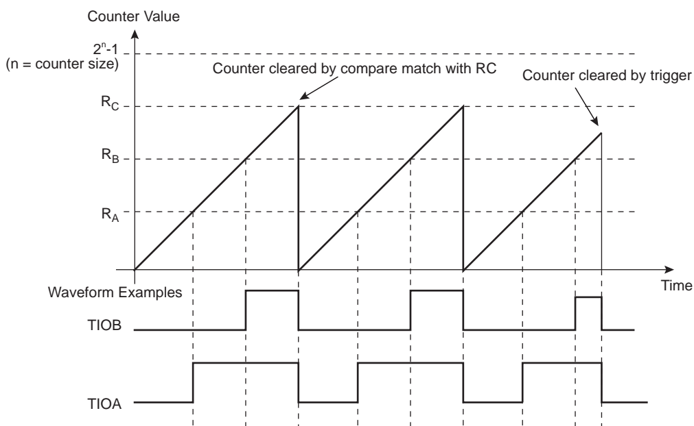
Figure 51-11. WAVSEL = 10 with Trigger
