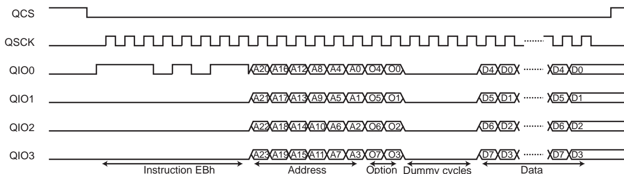
Figure 47-8. Instruction Frame
