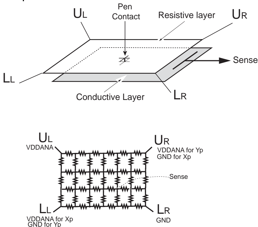
Figure 62-17. 5-Wire Principle
