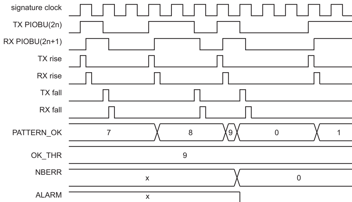
Figure 61-9. Dynamic Signatures: Resetting Error Counter After Receiving a Sufficient Number of Good Patterns
