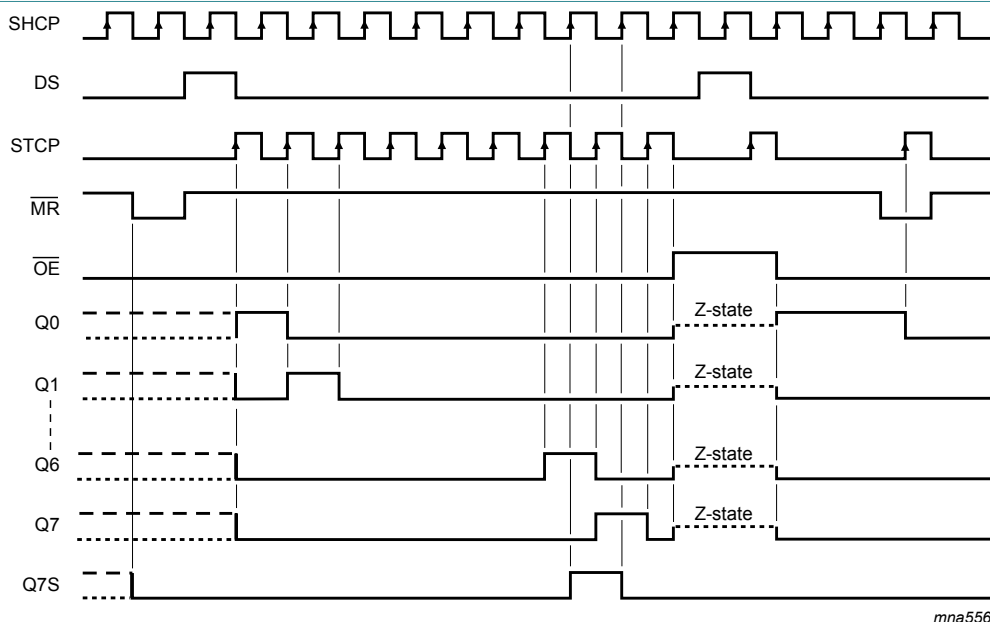
Figure 7. Timing diagram
