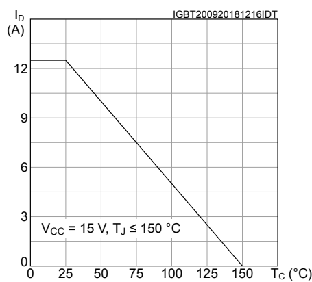
Figure 13. I_D vs temperature
