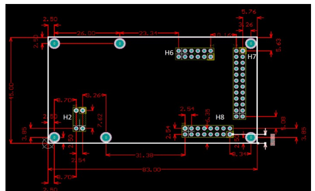
Figure 3: SM2400-EV1Mx-x Top View
