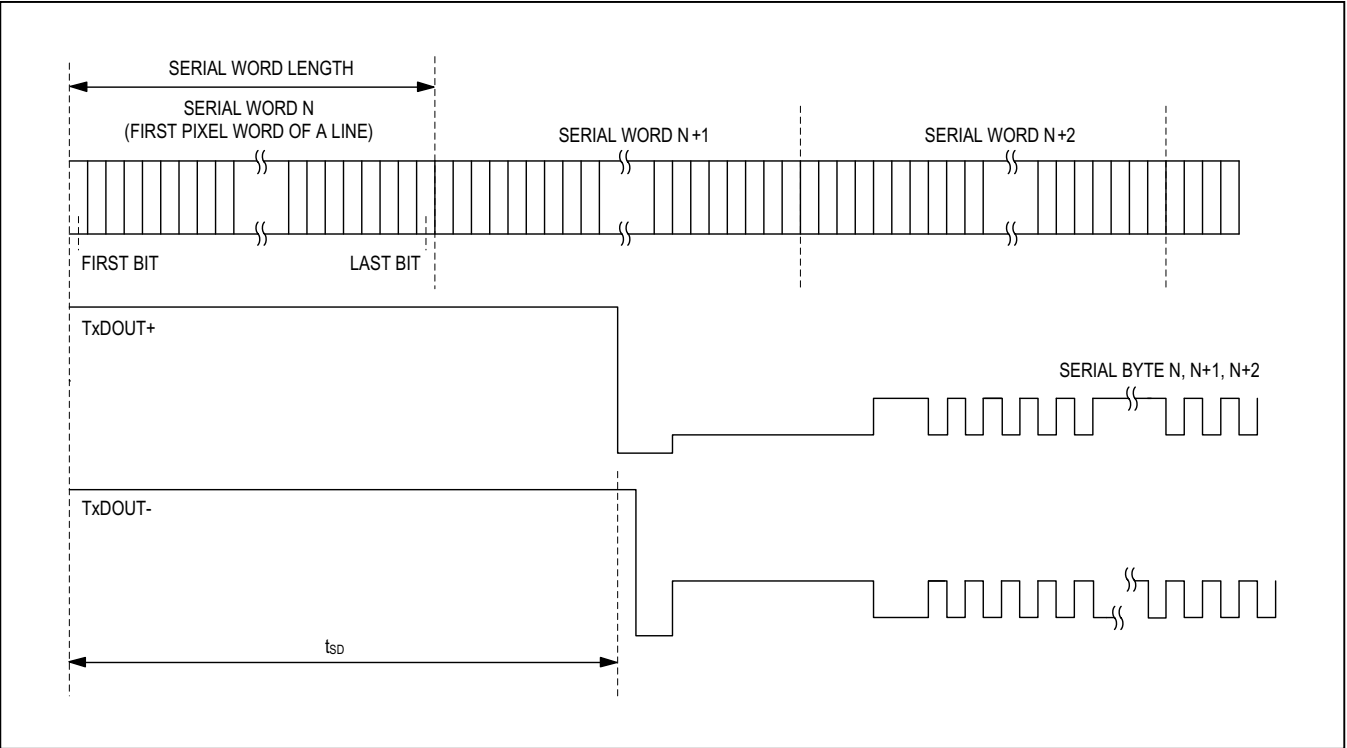
Figure 8. Deserializer Delay
