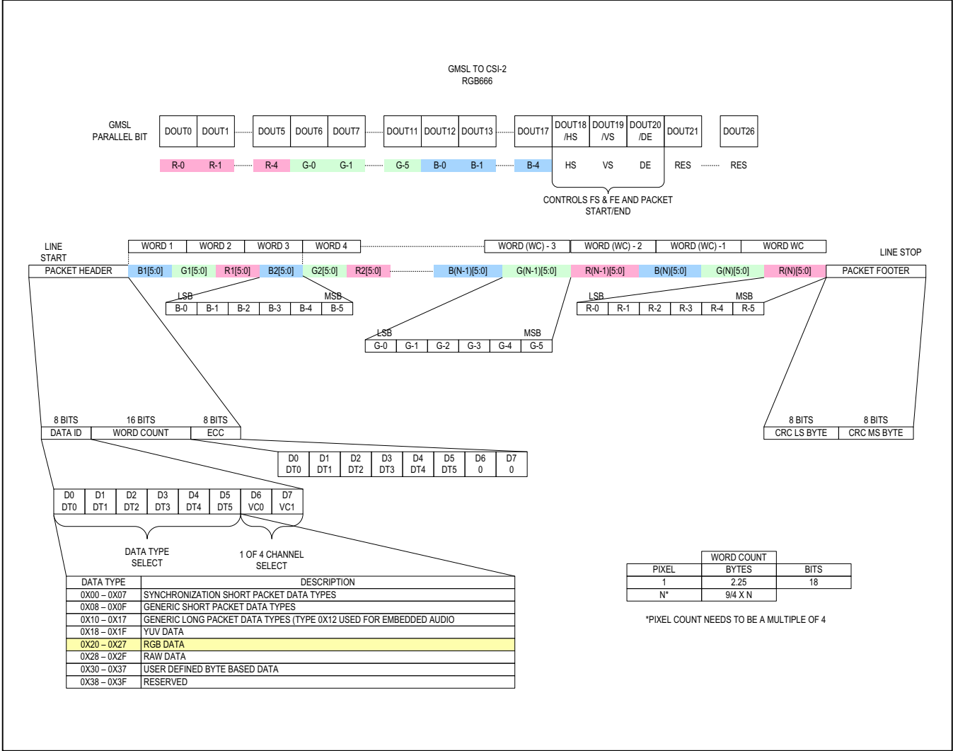
Figure 19. RGB666 Output
