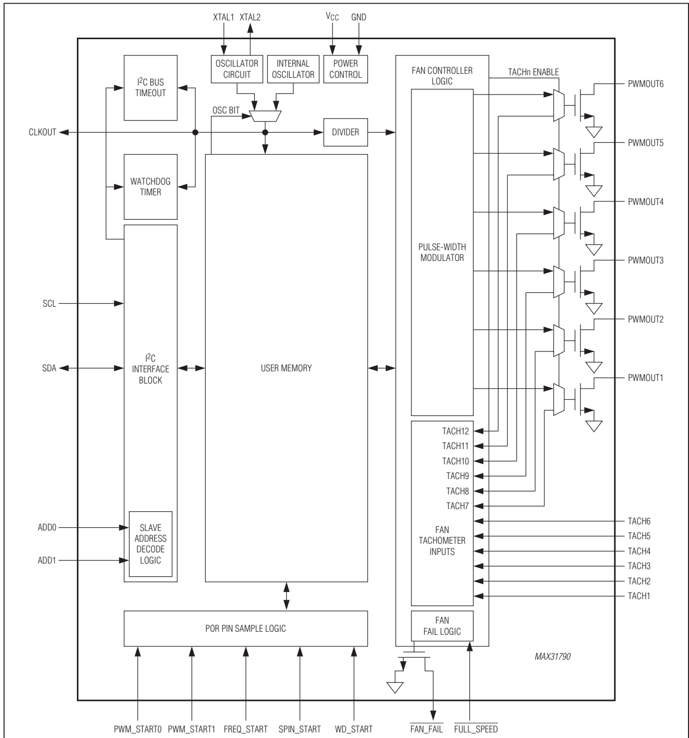
Block Diagram
