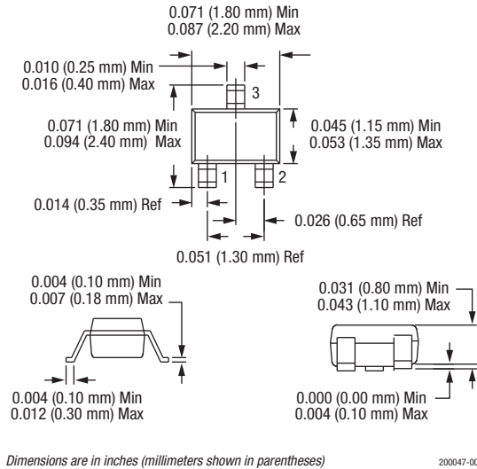
Figure 5. SC-70 Package Dimension Drawing
