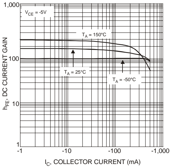
Fig. 5 DC Current Gain vs. Collector Current
