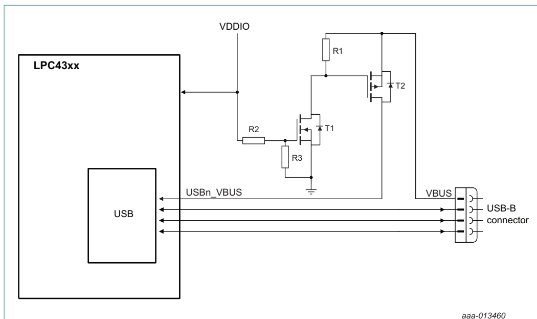
Fig 47. USB interface for USB operating in OTG mode
