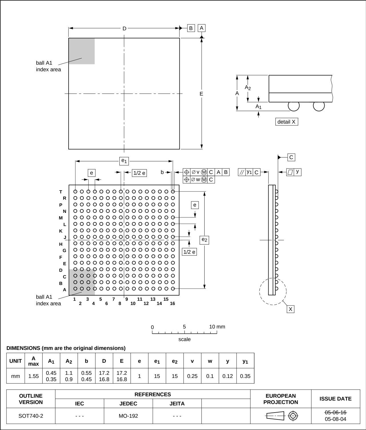
Fig 53. Package outline LBGA256 package
