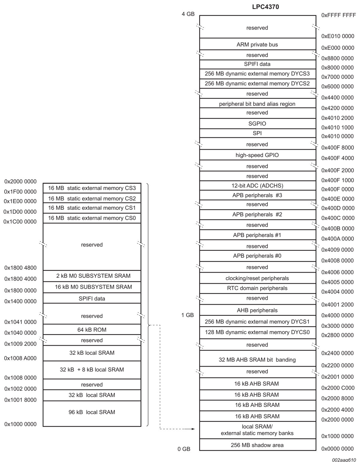
Fig 5. LPC4370 Memory mapping (overview)
