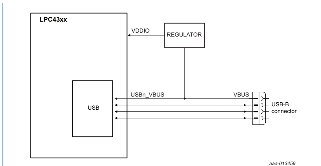
Fig 46. USB interface on a bus-powered device
