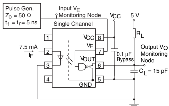
Figure 3. Single Channel Test Circuit for t_{EHL} and t_{ELH}
