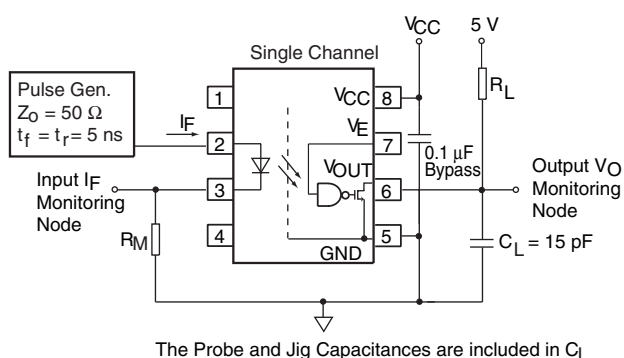
Figure 1. Single Channel Test Circuit for t_{PLH} , t_{PHL} , t_r and t_f
