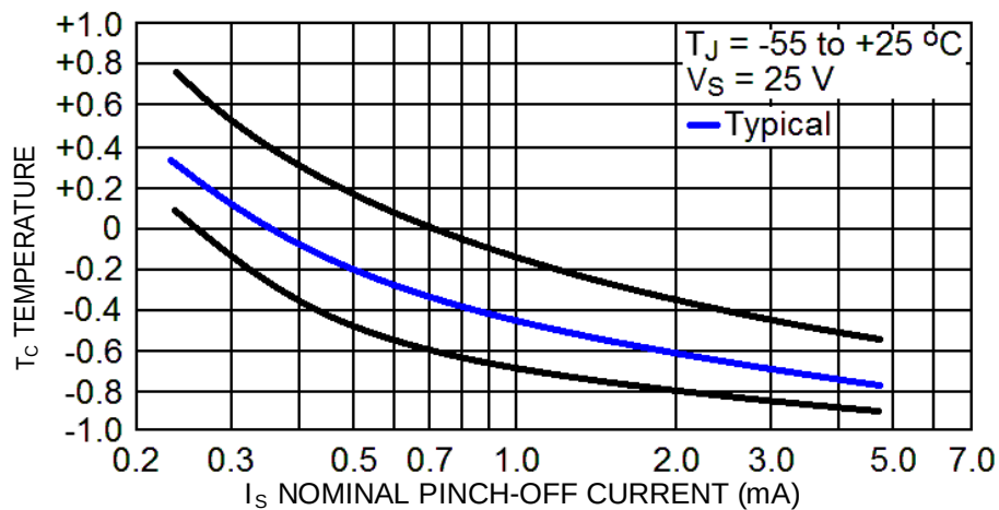
FIGURE 3 – TEMPERATURE COEFFICIENT
