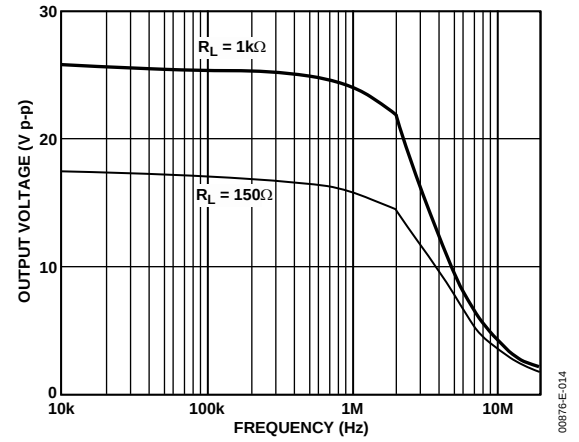
Figure 16. Large Signal Frequency Response; G = +2
