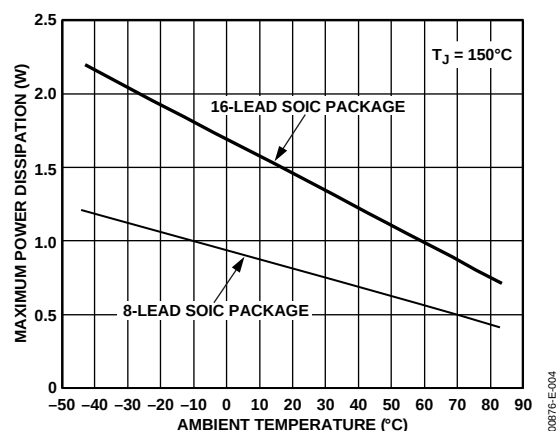
Figure 5. 16-Lead SOIC
