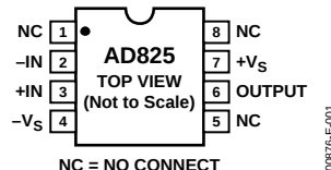
Figure 1. 8-Lead Plastic SOIC (R-8) Package
