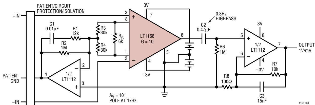
Figure 8. Nerve Impulse Amplifier
