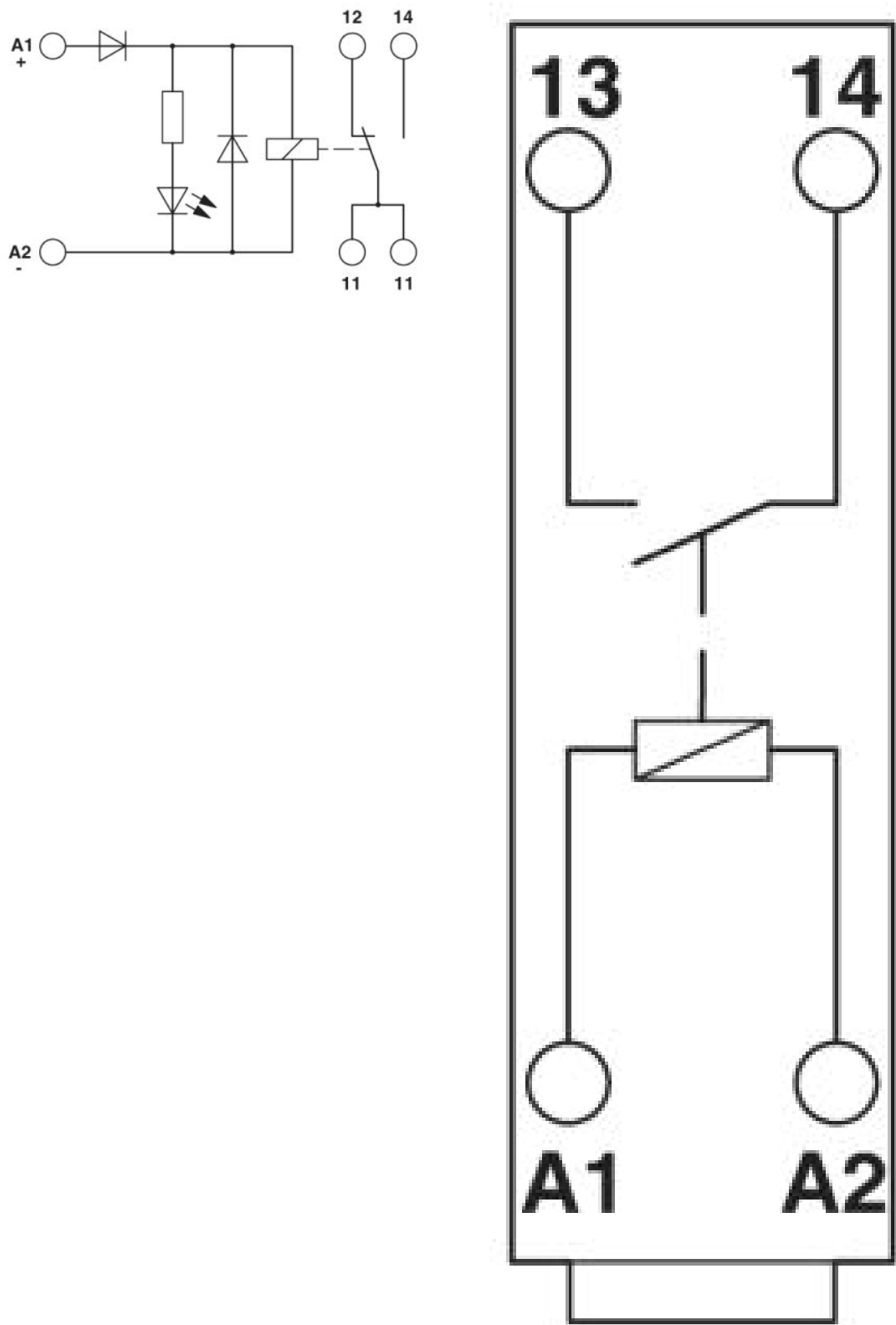
Circuit diagram
