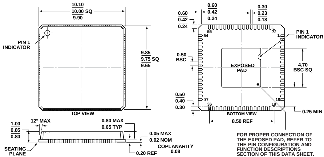
Figure 43. 72-Lead Lead Frame Chip Scale Package [LFCSP_VQ] 10 mm × 10 mm, Very Thin Quad (CP-72-1) Dimensions shown in millimeters
