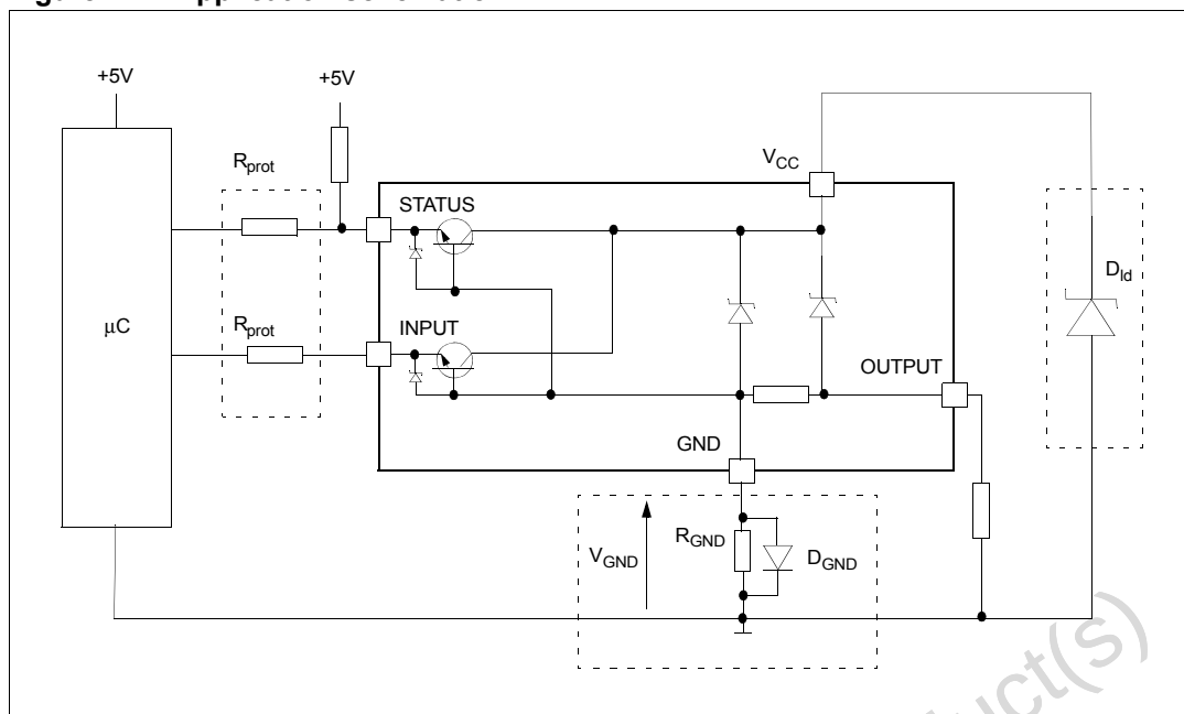
Figure 7. Application schematic
