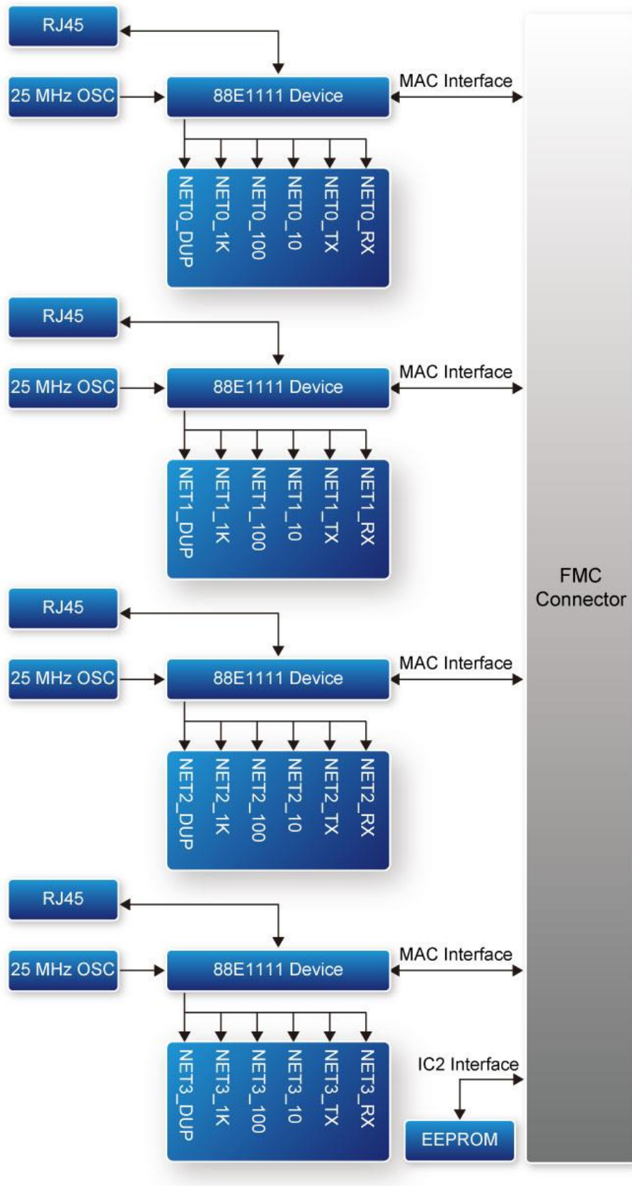
Figure 2-3 Block Diagram of NET-FMC Board
