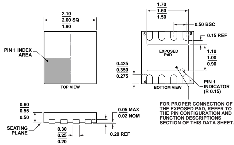
Figure 21. 8-Lead Lead Frame Chip Scale Package [LFCSP] 2.00 mm x 2.00 mm Body, and 0.55 mm Package Height (CP-8-10) Dimensions shown in millimeters
