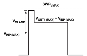
Figure 74. Clamping Waveform
