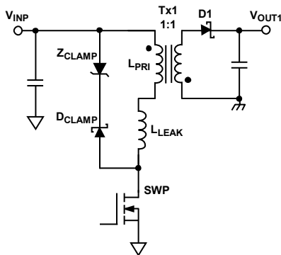
Figure 73. Diode Zener Diode Clamp
