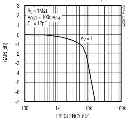
MAX4470/MAX4471/MAX4472 SMALL-SIGNAL GAIN vs. FREQUENCY
