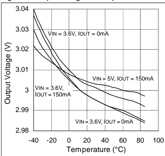
Figure 8. Output Voltage vs. Temperature
