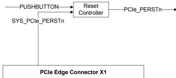
Figure 4: Board Reset
