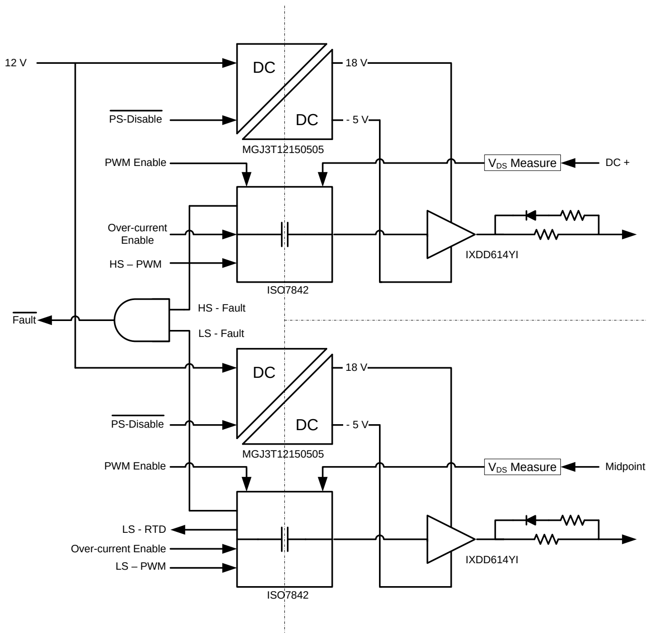
Fig 1. Block Diagram
