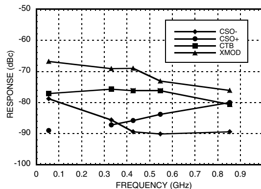
CSO / CTB / XMOD @ +15 dBmV input, 133 channels (Analog)
