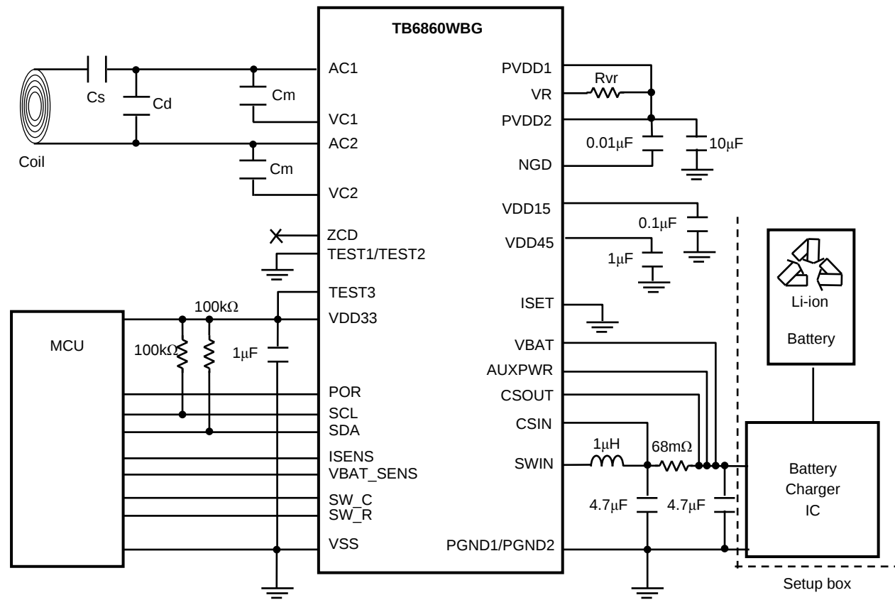
Figure 13.2 Feed mode
