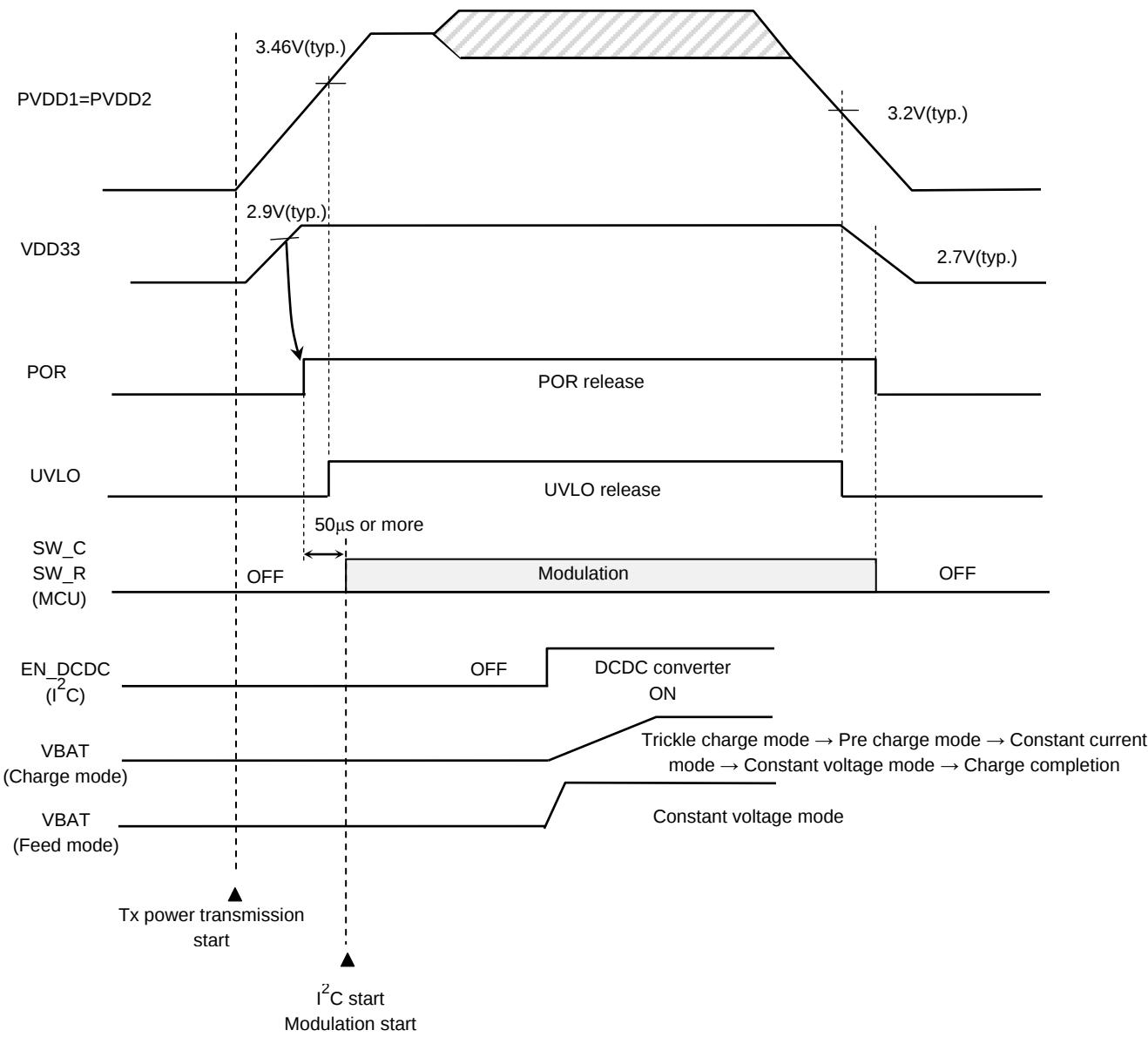
Figure 10.1 Start sequence
