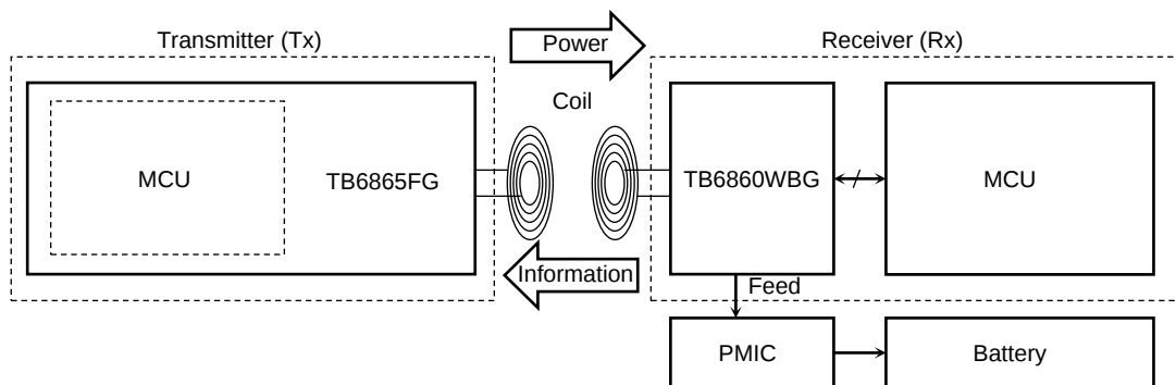
Figure 8.2 Feed mode
