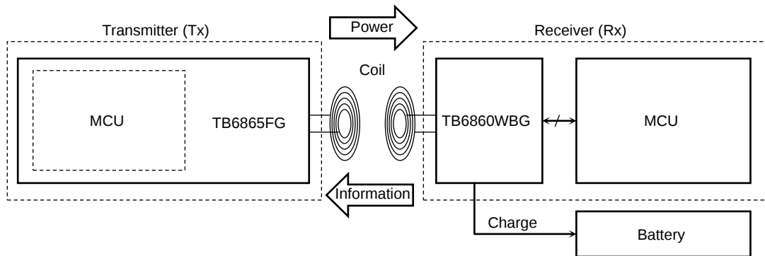
Figure 8.1 Charge mode
