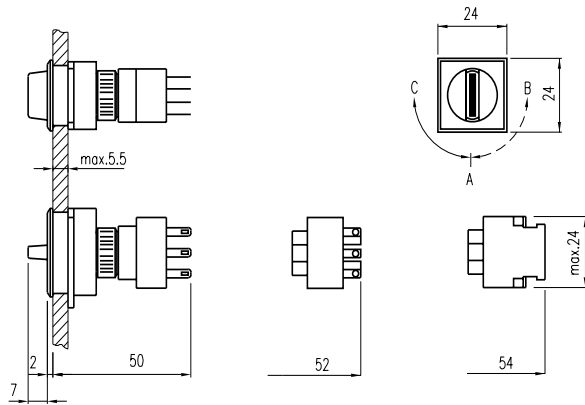
snap-action switching element with soldering-/plug-in element slow-make switching element with soldering-/plug-in terminal slow-make switching element with screw terminal
