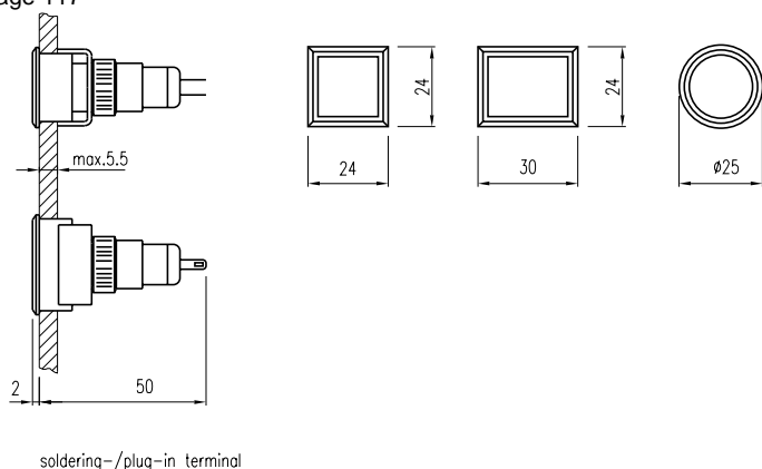
soldering-/plug-in terminal
