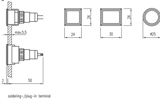
soldering-/plug-in terminal
