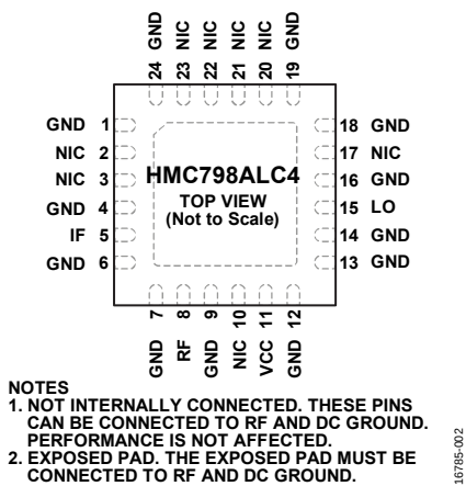
Figure 2. Pin Configuration
