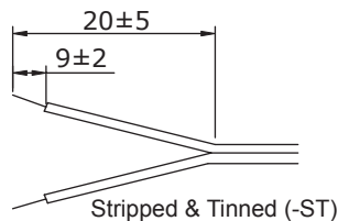
Stripped & Tinned (-ST)
