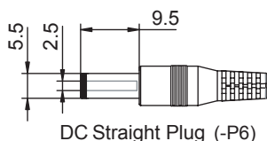
DC Straight Plug (-P6)
