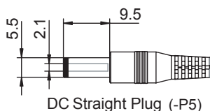
DC Straight Plug (-P5)
