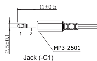
Jack (-C1)
