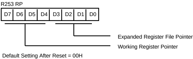
Figure 64. Register Pointer (F DH : Read/Write)
