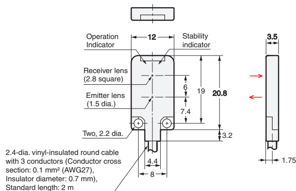
Mounting Holes
