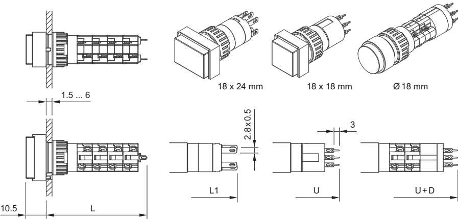
8 Illuminated pushbutton actuator page 6
