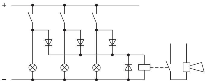
Alarm circuit from fault annunciation system
