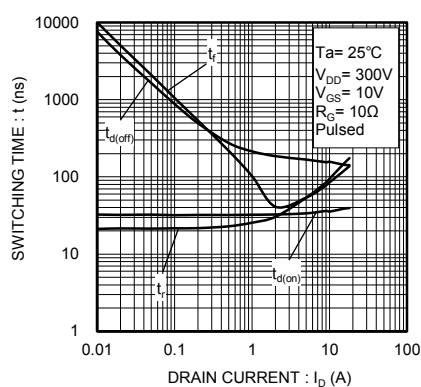
Fig.13 Switching Characteristics
