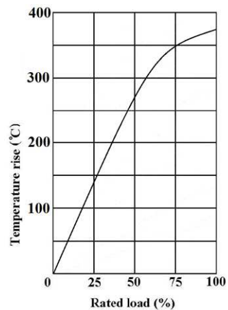
Temperature Rise Chart
