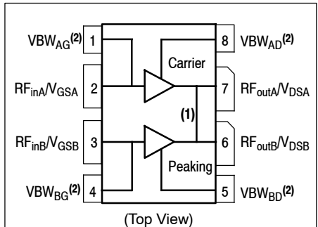
Figure 1. Pin Connections
