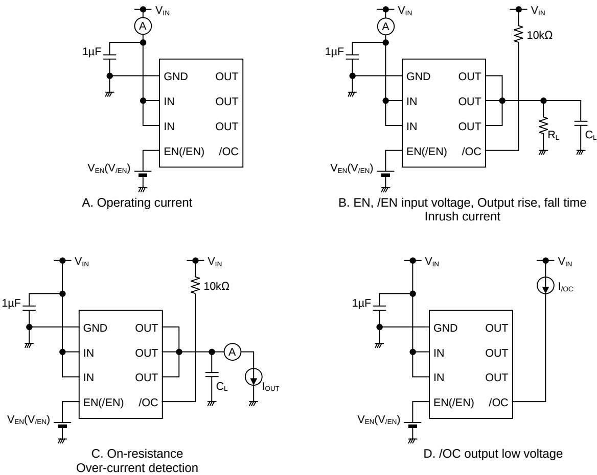
Figure 1. Measurement circuit
