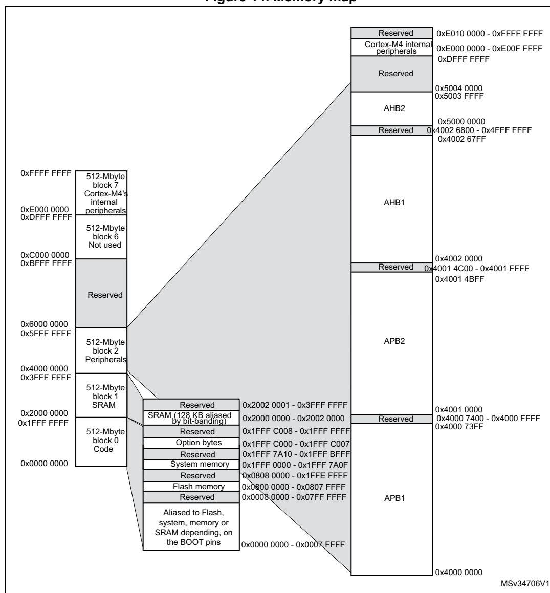
Figure 14. Memory map
