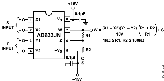
Figure 17. Connections for Variable Scale Factor
