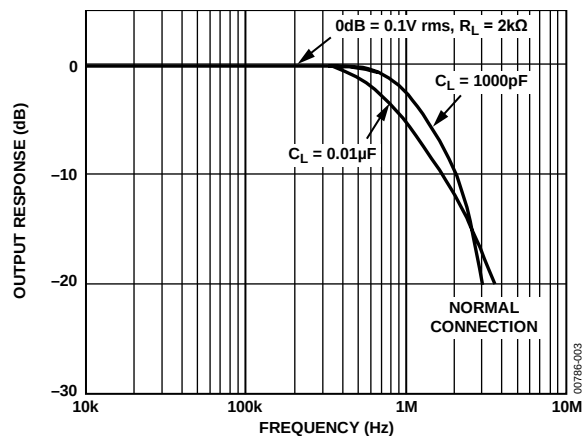
Figure 4. Frequency Response
