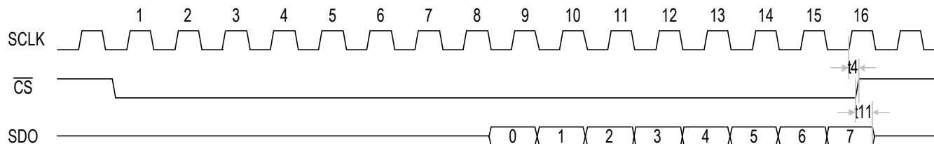
Figure - 34. Serial Interface Read Timing with CLKE = 1
