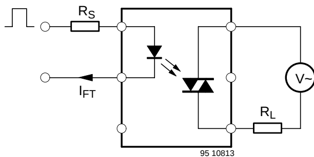
Figure 1. Test circuit for dv/dt_{cr} and dv/dt_{crp}
