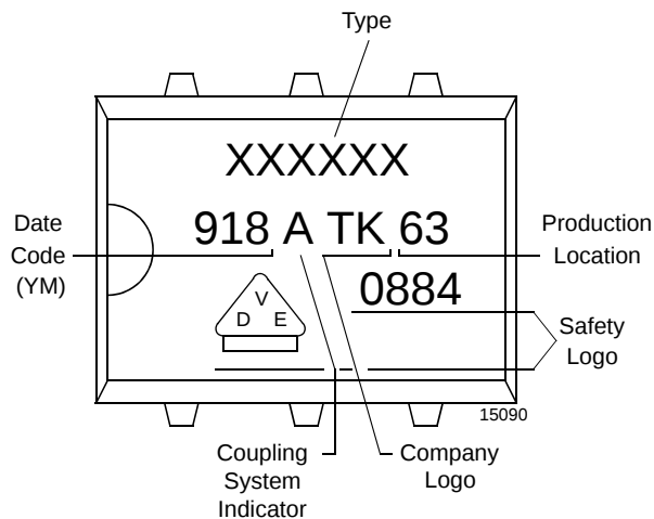
Figure 12. Marking example
