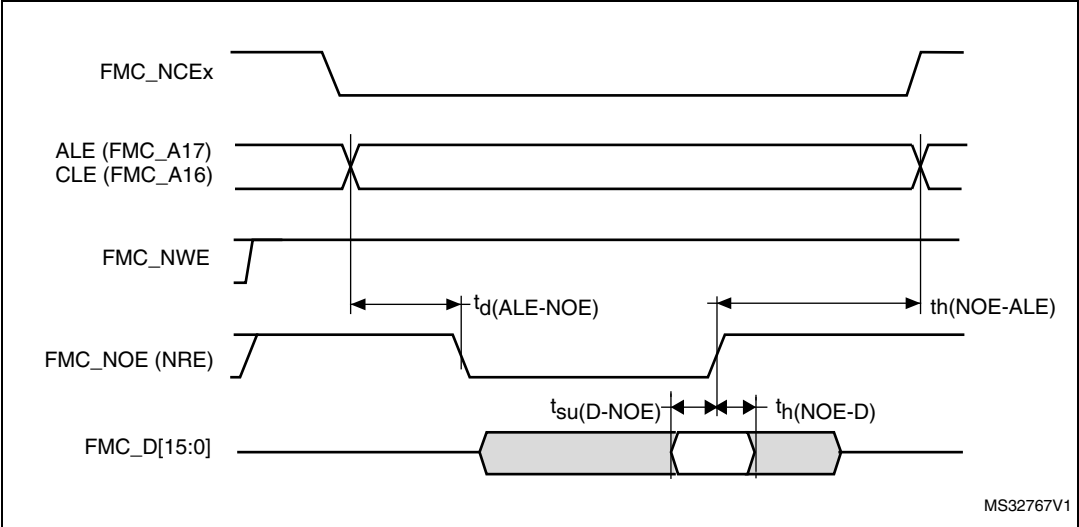
Figure 58. NAND controller waveforms for read access
