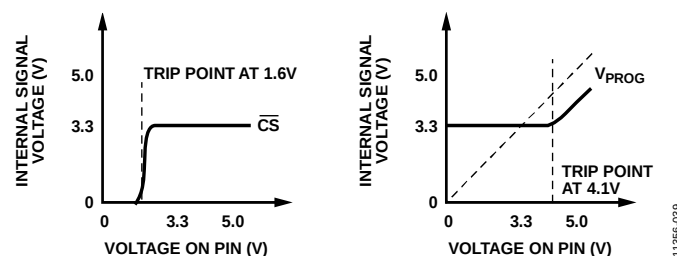
Figure 35. \overline{\text{CS}} Pin Function
