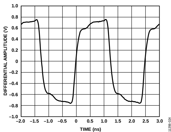
Figure 18. Output Waveform, HCSL (400 MHz)
