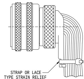
TYPICAL INSTALLATION
