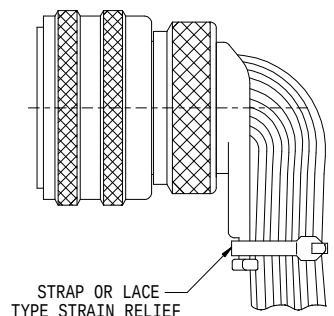
TYPICAL INSTALLATION
